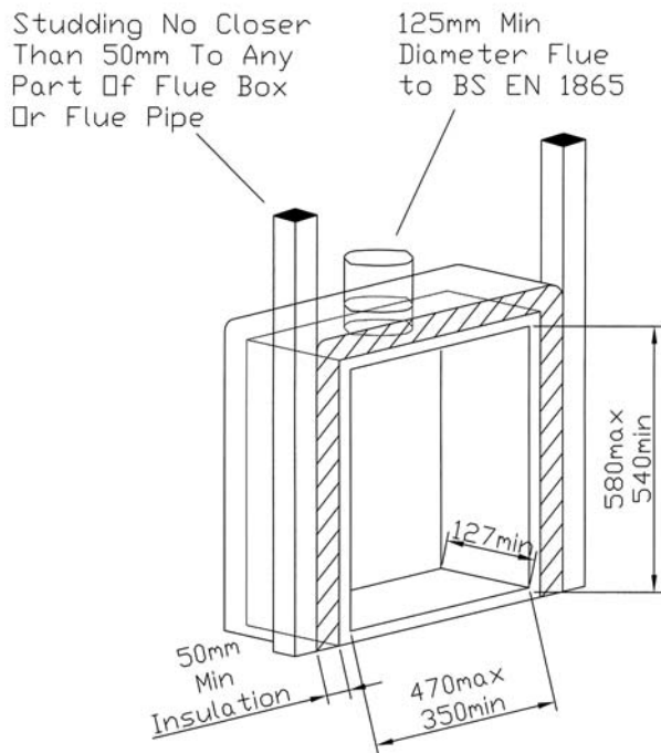
BS715 Shallow Flue Box Application
